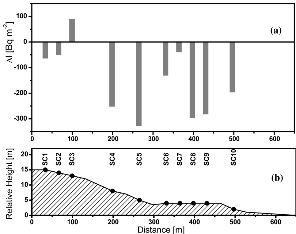
Fig. 6 \Delta I equal to difference between ^7\text{Be} soil inventory of each sampling point and the ^7\text{Be} soil inventory of the Reference Site ( 571 \pm 48 \text{ Bq m}^{-2} ) on June 17, 2017 (a); along the transect (b). The 0 m is taken at 1010 m a.s.l
