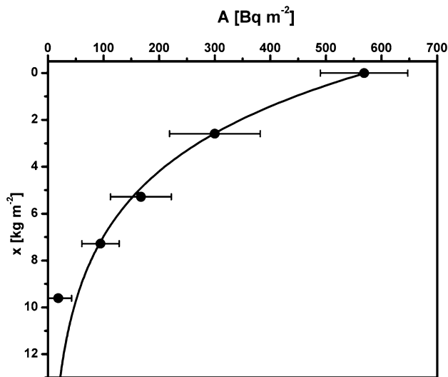
Fig. 5 Average ^7\text{Be} soil content A(x) [ \text{Bq m}^{-2} ] as a function of mass depth x [ \text{kg m}^{-2} ] (circles) in the Reference Site on June 17, 2017. Curve obtained by fitting with Eq. (2) (line). The error bars represent the standard deviation
